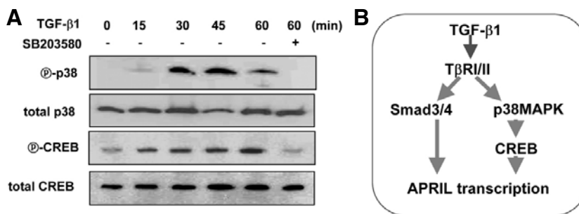
Fig. 5. TGF- \beta 1 induces p38MAPK and CREB phosphorylation. (A) Cells were stimulated with TGF- \beta 1 (1 ng/ml) as indicated. Cells were pre-incubated with 5 \mu M SB203580 for 1 h. Phosphorylated p38MAPK ( \textcircled{P} -p38), total p38MAPK, phosphorylated CREB ( \textcircled{P} -CREB), and total CREB were detected by Western blot. (B) Proposed mechanisms underlying TGF- \beta 1-induced APRIL expression in mouse macrophages.
