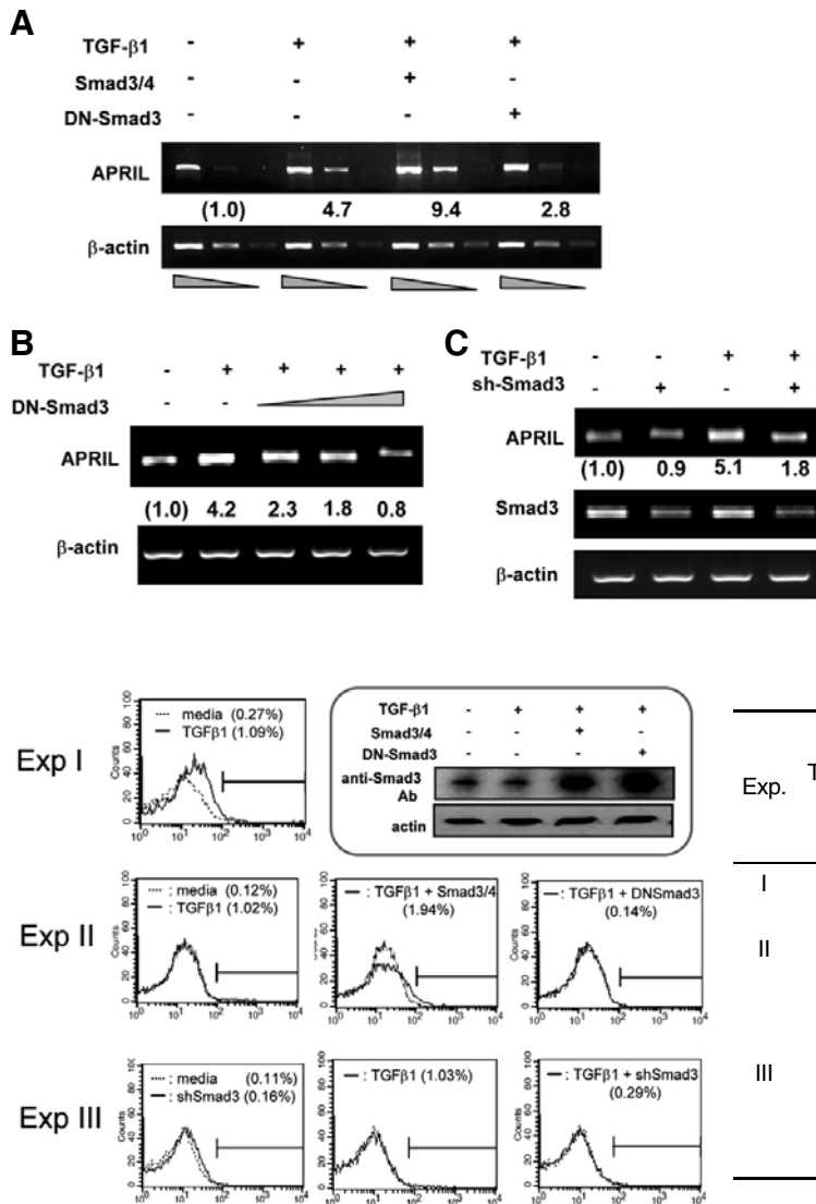
Fig. 3. Effects of TGF- \beta 1 and Smad3/4 on Surface APRIL Expression. P388D1 cells were transfected with Smad3/4 (each 2 \mu g), DN-Smad3 (8 \mu g) or Smad3 shRNA (2 \mu g) and incubated with TGF- \beta 1 (1 ng/ml) for 48 h. Surface APRIL expression was analyzed by FACS by using anti-APRIL antibody. Western blot was performed to detect the expression of transfected Smad3 (rounded box).
